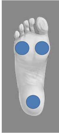
FIGURE 1: Position of factors under the sole of the foot (1st and 5th metatarsal-phalangeal joint region and heel).
